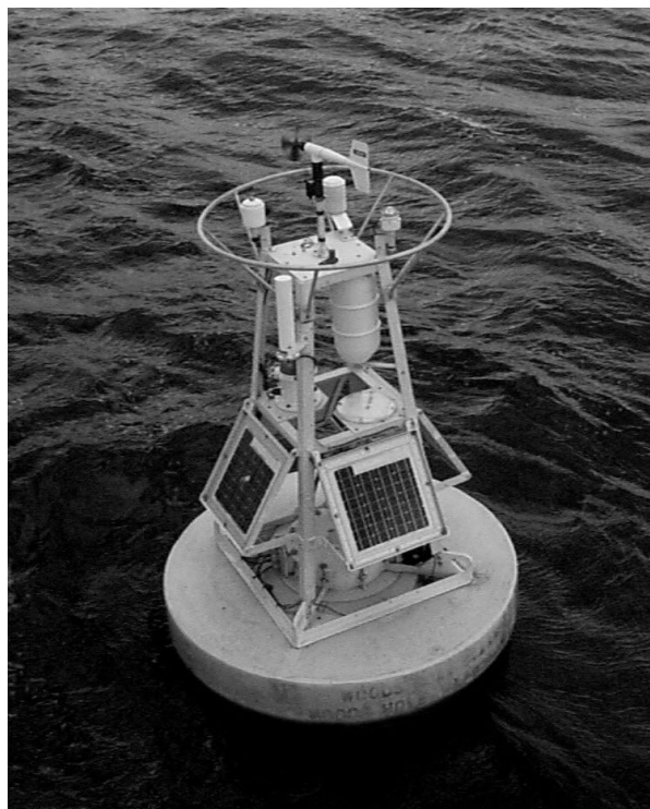
Figure 1. The GLOBEC buoy with meteorology sensors visible on the top of the tower. The R.M. Young Anemometer is highest; behind it is the Gill radiation shield holding the Rotronics air temperature and relative humidity sensor. On the left is the Eppley long-wave radiation; on the right is the Eppley short-wave radiation sensor. The small dark sensor on the front of the top plate of the tower is the LiCor cosine PAR sensor.
